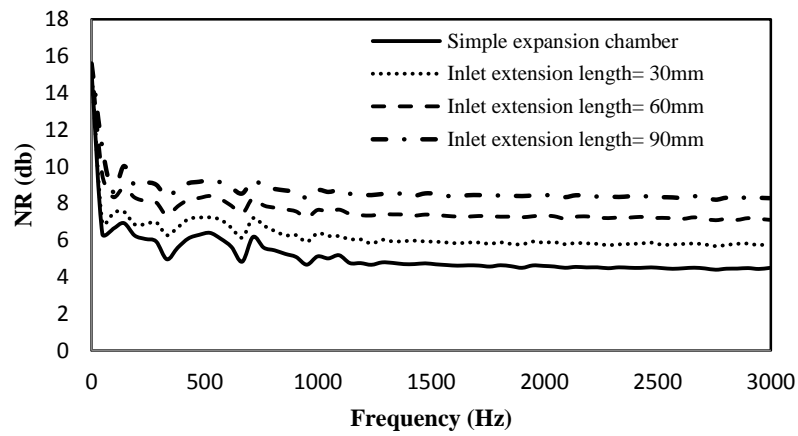
Fig 12: NR of simple and extended mufflers.
