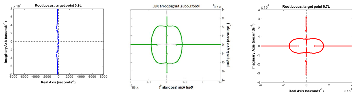
Fig. 10: Root locus diagrams for different target pints on the cantilever
