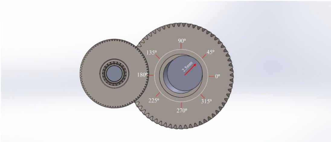
Fig.11. Front view of misalignment on the inclined plane (45 degrees) in SolidWorks
