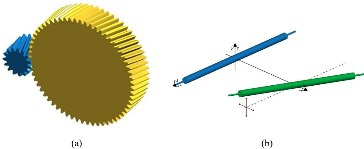
Fig.6. Output and second idler shaft: a) gears, b) misaligned axes simulated in KISSsoft
