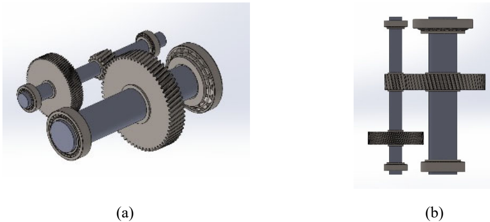
Fig.4. Aligned positions of the output shaft and second idler shaft: a) Isometric view, b) Top view
