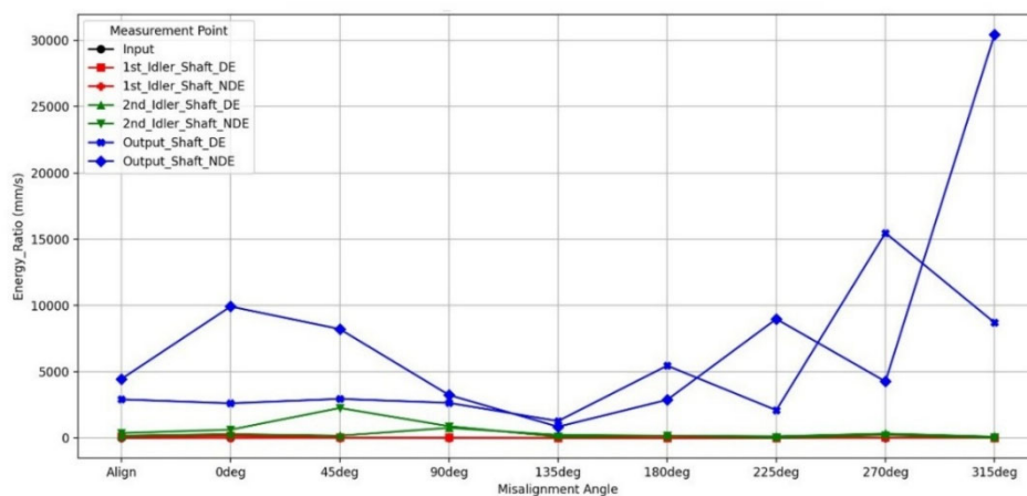
Fig.14. Variation of the energy ratio feature at different misalignment angles for the acceleration signal.
