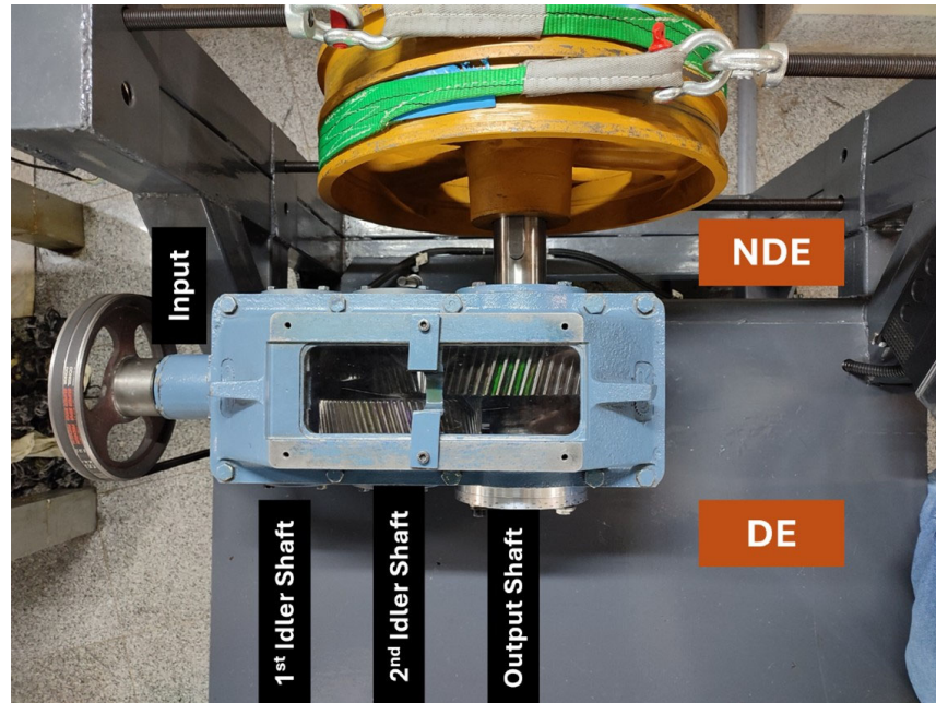
Fig.9. Measurement points
