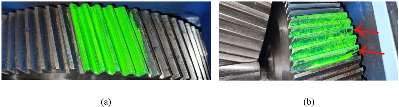
Fig.2. Blue check test between output and second idler shaft gears: a) Before engagement, b) After engagement
